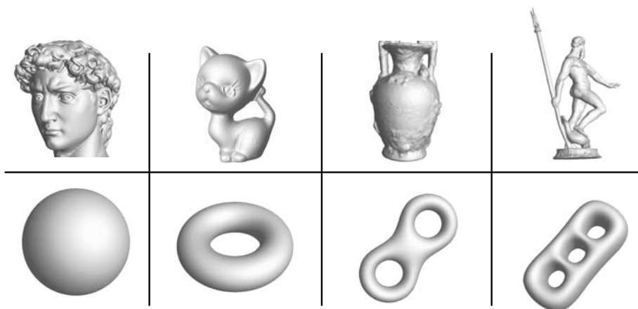
1.3—Surfaces of genus 0, 1, 2, and 3; the term genus refers to the number of holes.
