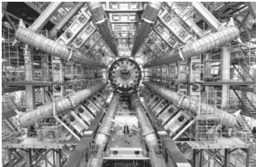
12.2—Experiments at the Large Hadron Collider (LHC) at the CERN lab in Geneva could find hints of extra dimensions or the existence of supersymmetric particles. Apparatus from the LHC's ATLAS experiment is shown here. (Courtesy of CERN)
