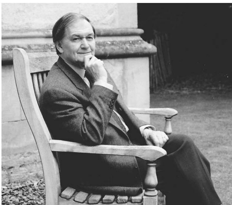
3.10b—Oxford University mathematician Roger Penrose (© Robert S. Harris [London])
