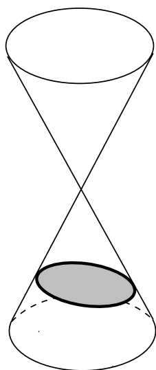
Ellipse
